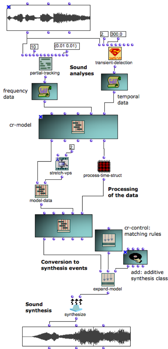
Fig. 14. Example of a full sound analysis/processing/synthesis process carried out in OpenMusic: sound descriptions are obtained from analysis tools, processed in the compositional framework, and converted back to synthesis parameters in order to generate other sounds.
