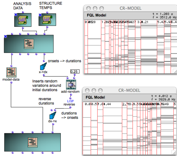
Fig. 6. cr-model time processing: the durations of the initial time structure are reversed and subjected to random variations.
