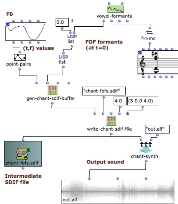
Figure 2. OM-Chant: Generation of SDIF data for the control of CHANT in OpenMusic.
